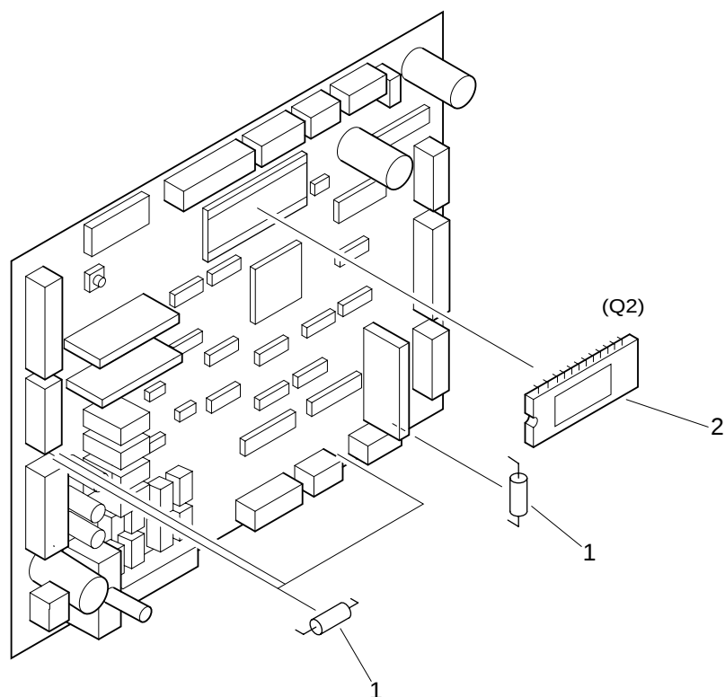
FIGURE T91 SADDLE CONTROLLER PCB ASS'Y (FINISHER-C2/H2)
