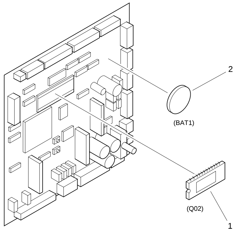
FIGURE T90 FINISHER CONTROLLER PCB ASSEMBLY
